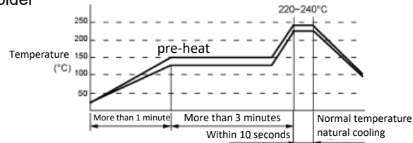
Reflow Soldering Recommended Conditions
