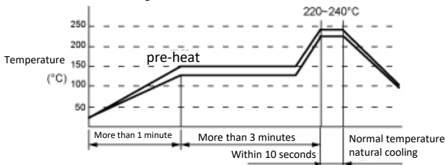
Reflow Soldering Recommended Conditions
